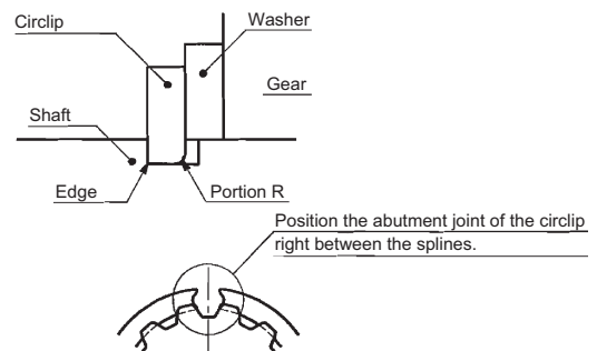
B Detail of installation of circlip
