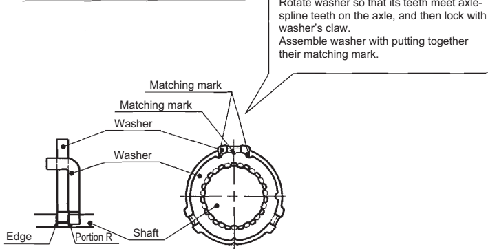
A Detail of installation of washer
